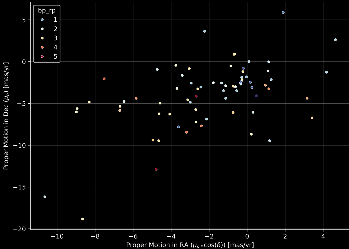
APOGEE DR17 Field: [001-01-O] Proper Motion Diagram (n= 71)
