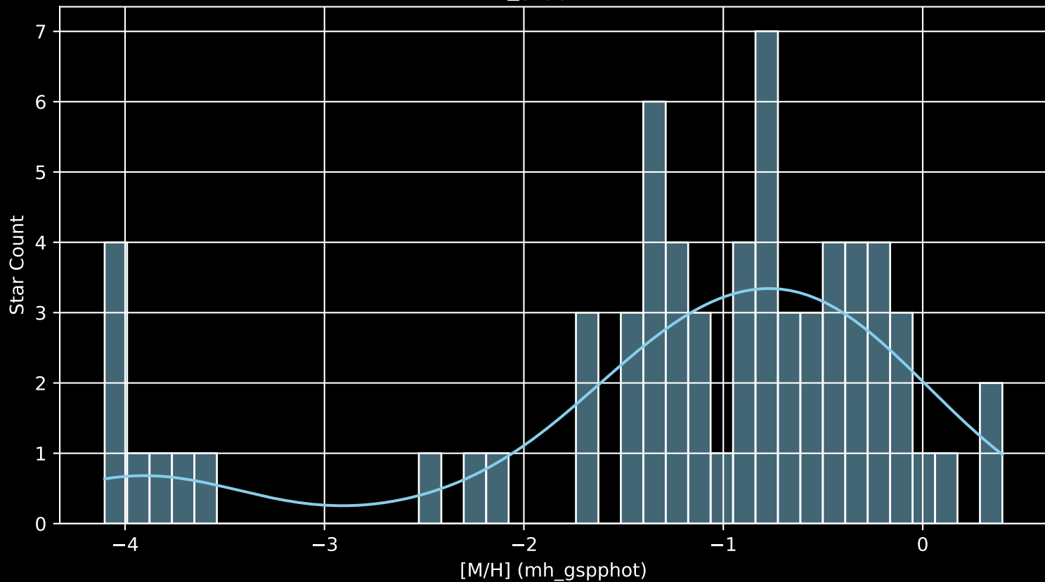
APOGEE DR17 Field: [001-01-O [M/H] (mh_gspphot) (n= 67)
