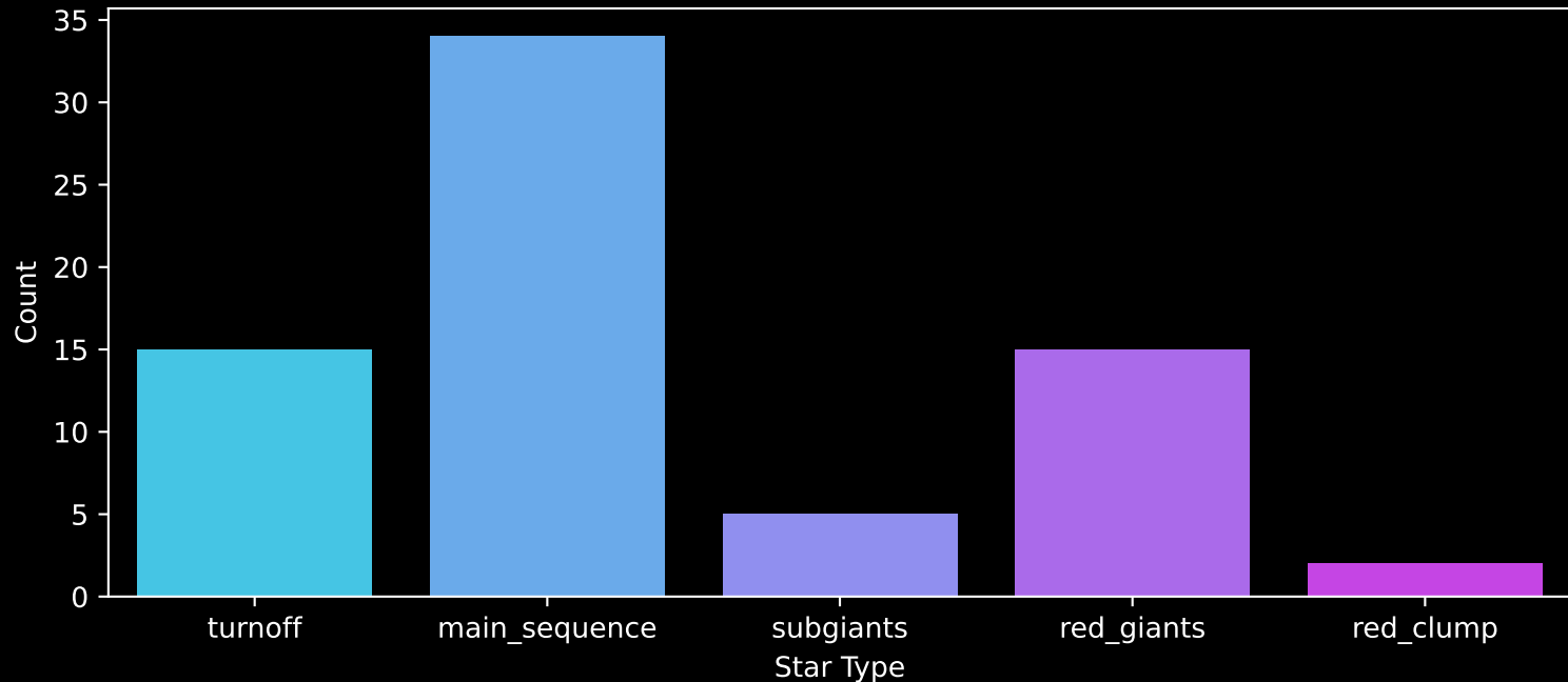
APOGEE DR17 Field: [001-01-O] Count plot of Star Type
