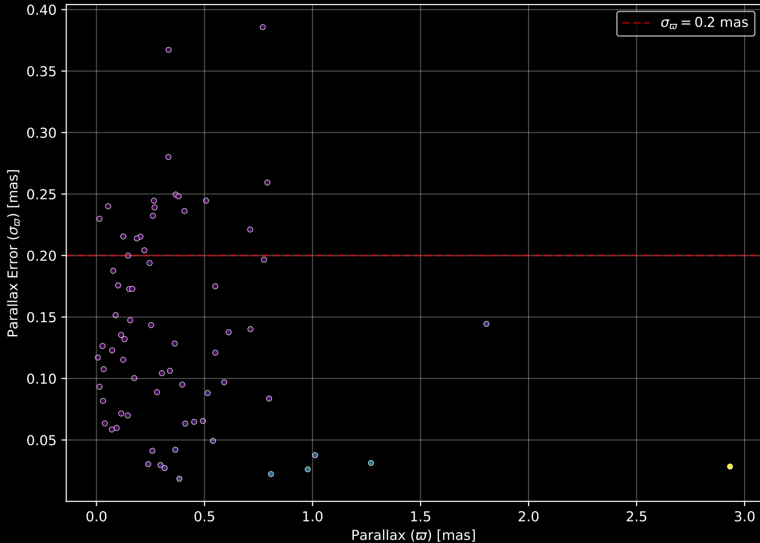
APOGEE DR17 Field: [001-01-O] Parallax Quality (n= 71)
