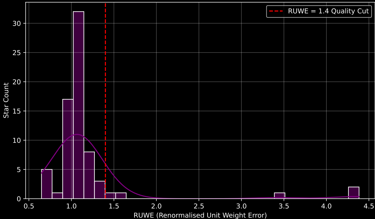
GAPOGEE DR17 Field [001-01-O] RUWE Distribution (n= 71)
