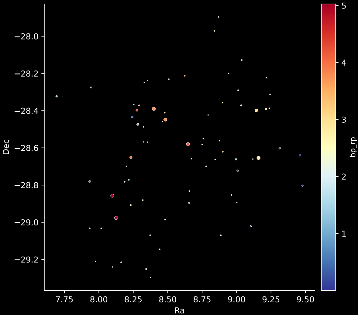
APOGEE DR17 Field: [001-01-O] Stars: 71
