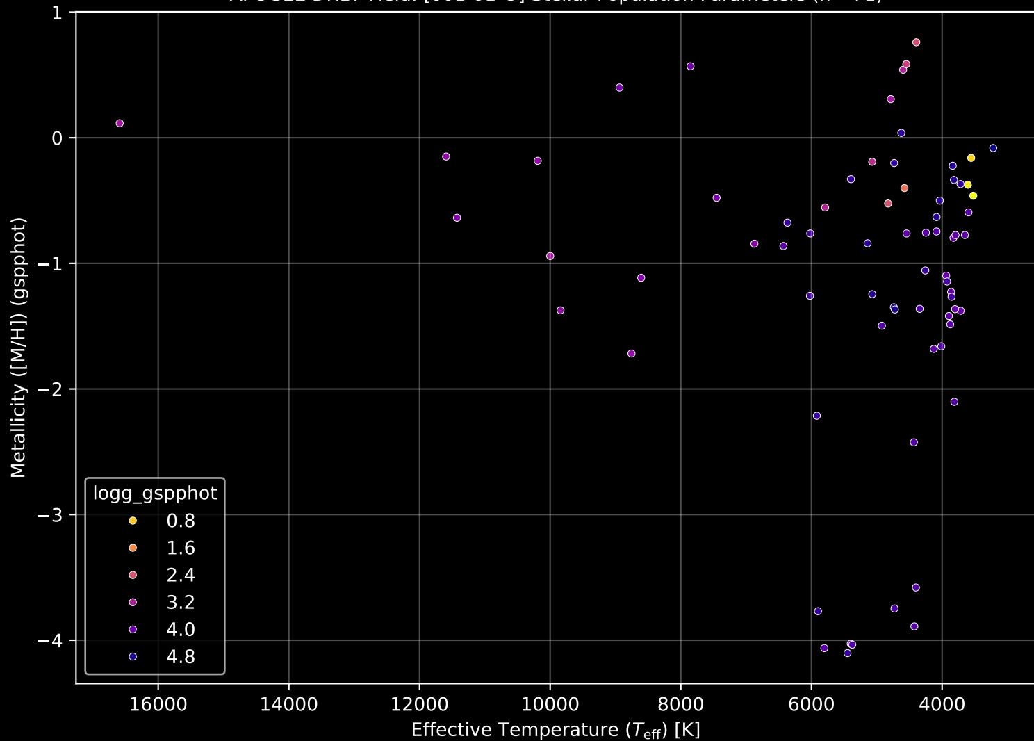
APOGEE DR17 Field: [001-01-O] Stellar Population Parameters (n= 71)
